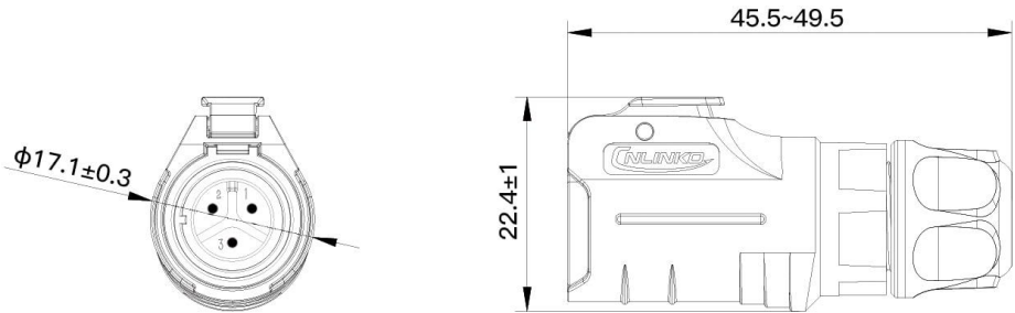
Plug
