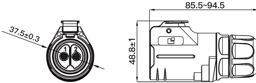
Female Plug
