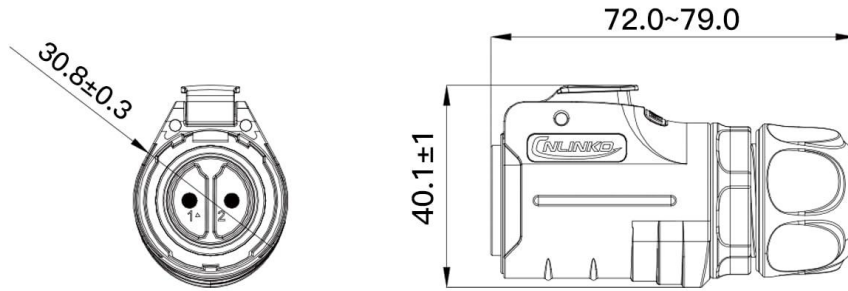
Female Plug
