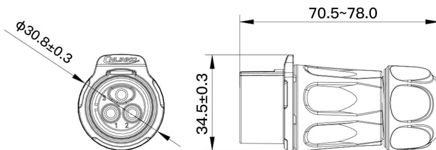
Female Plug
