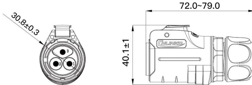
Female Plug
