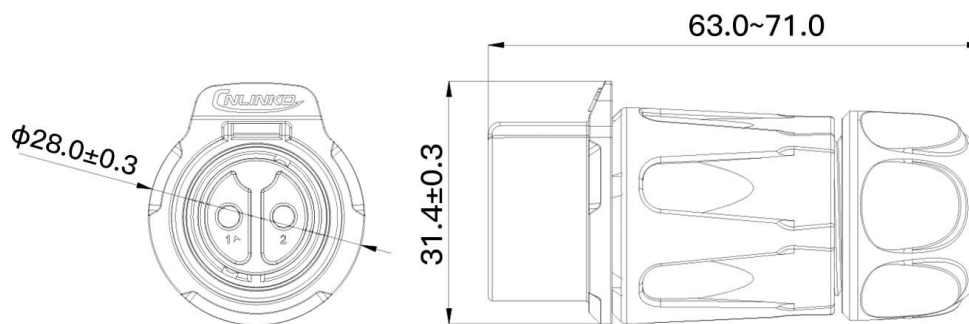
Female Plug
