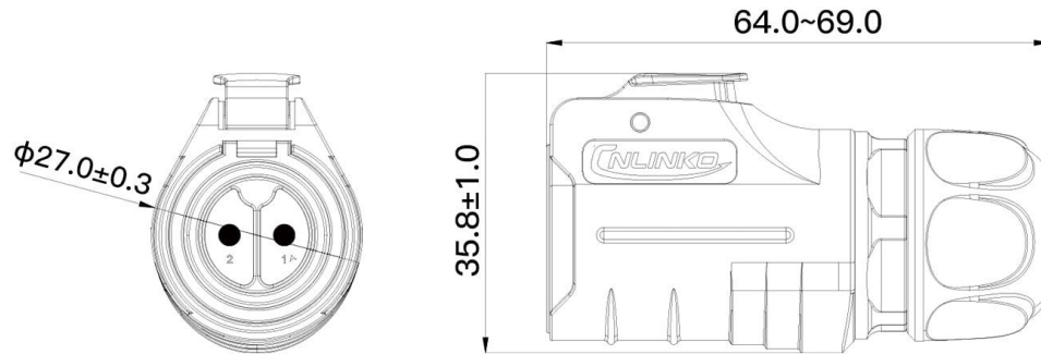
Male Plug
