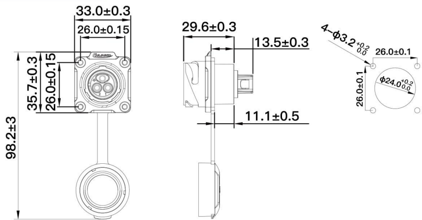
Four-Hole Socket
