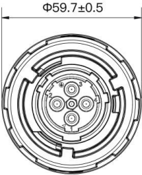
Female Mating Plug
